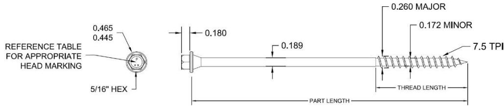
Figure 1: TimberLOK® Fastener
